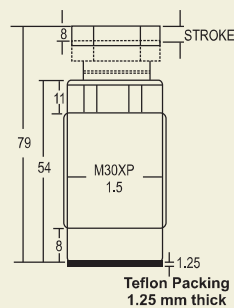
Spring Advance Threaded Body Type SP-16A
